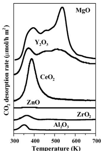
Fig. 1. TPD profiles of CO 2 on oxides with different acid-base properties. CO 2 adsorption at 298 K, 10 K/min heating rate.
